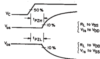
Figure 5-6. Turn-On Propagation Delay-control Input.
