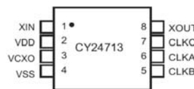
Figure 1. CY24713, 8-Pin SOIC
