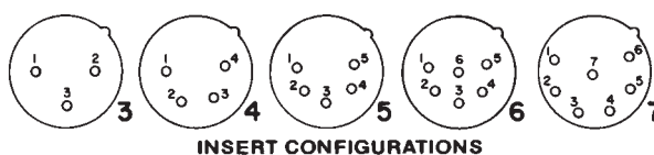
FACE VIEW OF PIN (MALE) INSERTS
