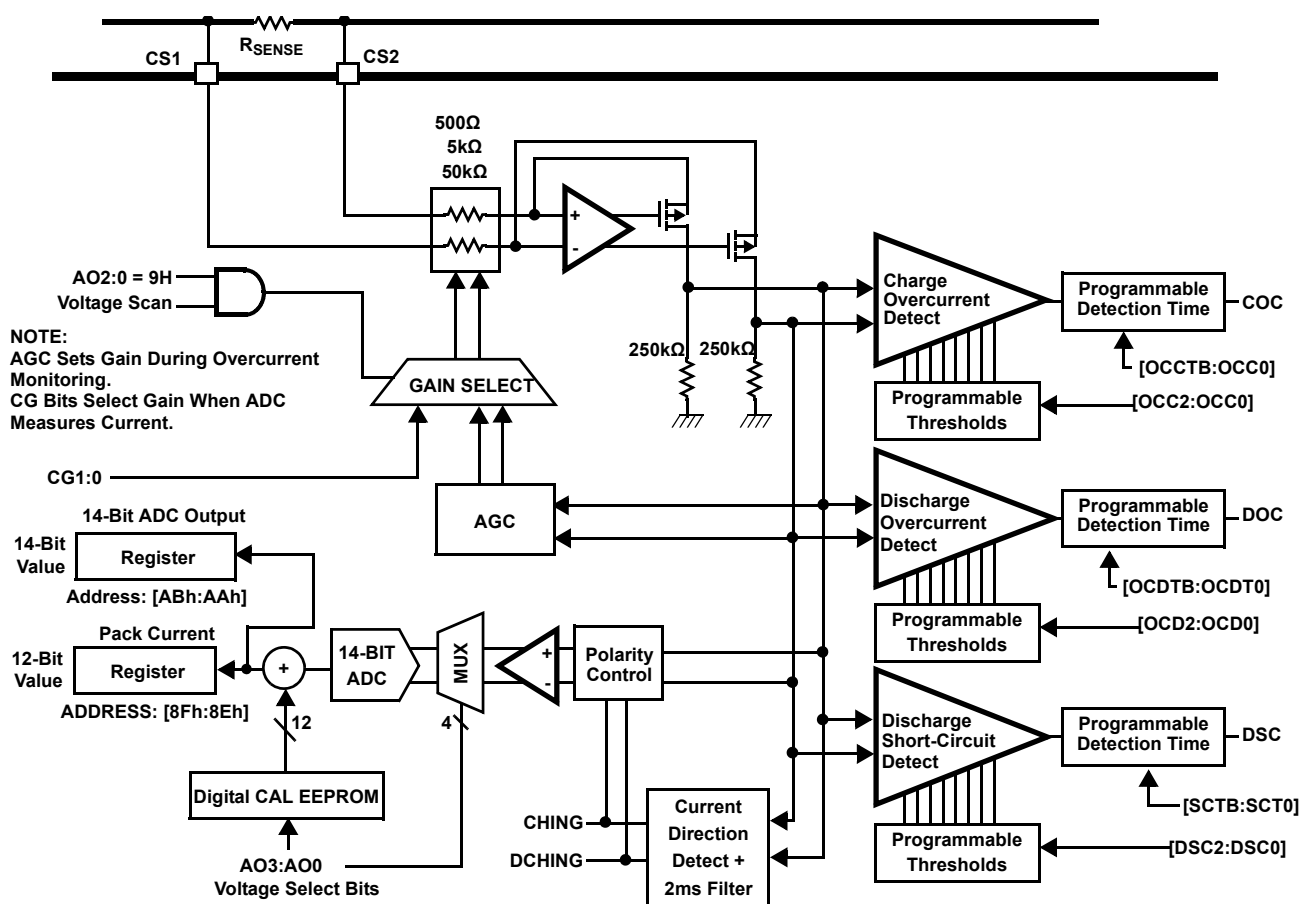
Figure 51. Current Sense
