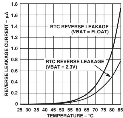
TPC 3. VRTC Reverse Leakage Current vs. Temperature
