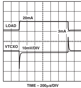
TPC 9. VTCXO Load Step
