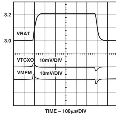
TPC 6. Line Transient Response, Maximum Loads
