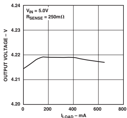
TPC 22. Charger V_{OUT} vs. I_{LOAD} ( V_{IN} = 5.0\text{ V} )
