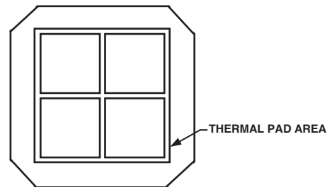
Figure 9. LFCSP Paste Mask Pattern
