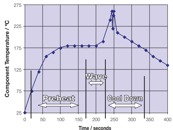
Recommended Soldering Profiles
