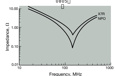
Variation of Impedance with Ceramic Form| Impedance vs. Frequency| 1000 pF - C0G (NP0) vs. X7R | 0805
