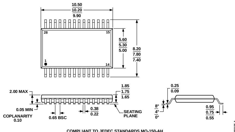
Figure 28. 28-Lead Shrink Small Outline Package [SSOP] (RS-28)
