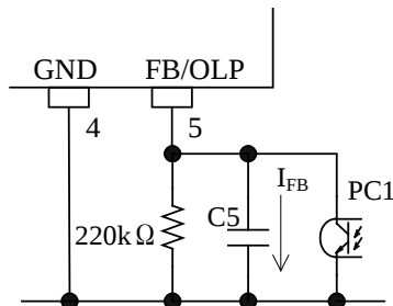
Figure 9-31 FB/OLP pin peripheral circuit (without latched operation)
