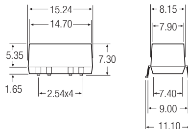
6 PIN Dual SMD Package
