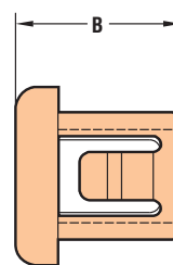
SINGLE PANEL THICKNESS DESIGN
