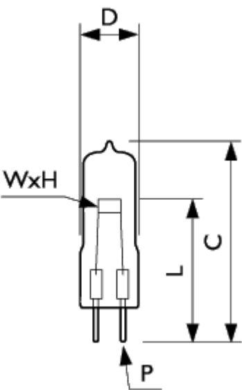
XHMPSEFF G6.35/GY6.35
