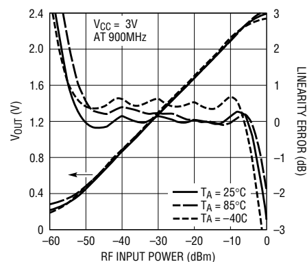
Output Voltage vs RF Input Power
