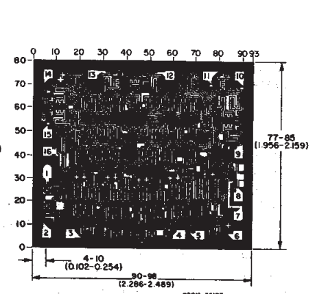
Dimensions and pad layout for CD4056BH.
