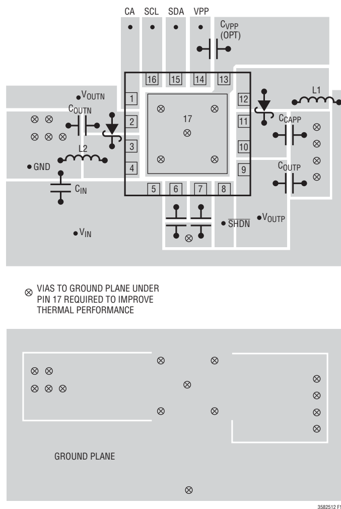
Figure 12. Suggested Component Placement (Not to Scale)
