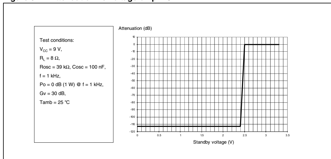
Figure 32. Attenuation vs voltage on pin STBY
