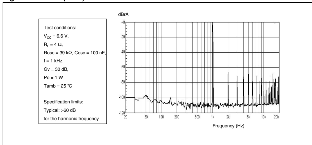
Figure 10. FFT (-60 dB)
