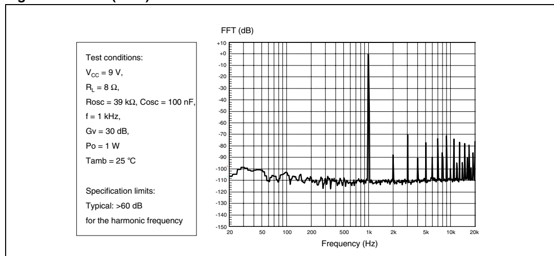
Figure 24. FFT (0 dB)
