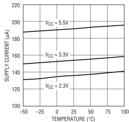
I_{CC2} Enabled Current vs Temperature
