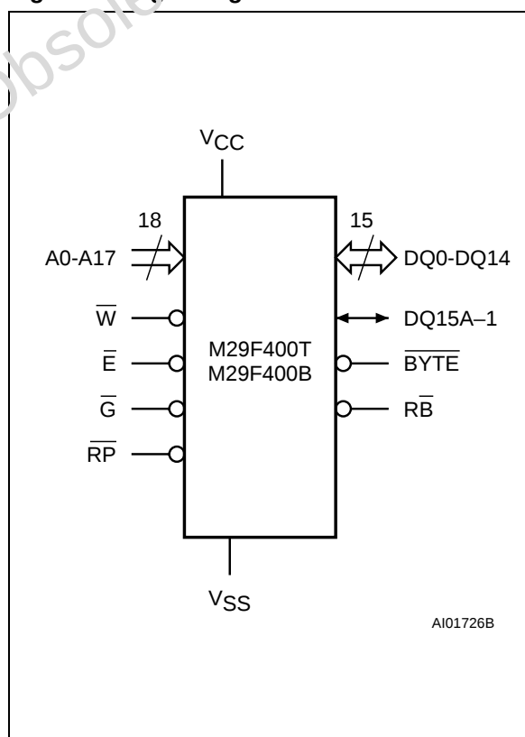
Figure 1. Logic Diagram
