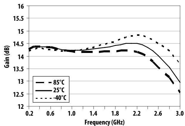
Figure 15. Gain over Frequency and Temperature
