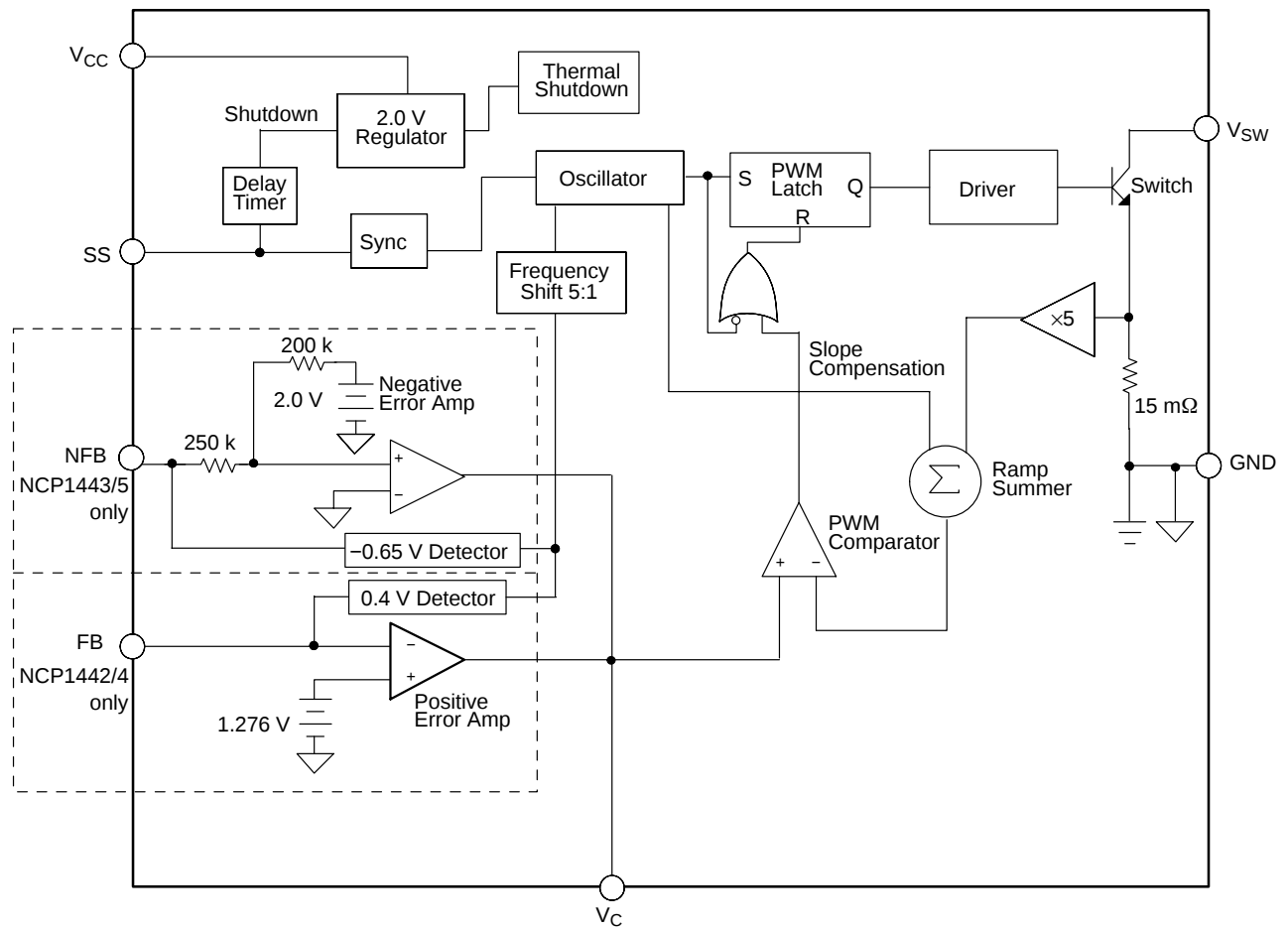
Figure 2. Block Diagram
