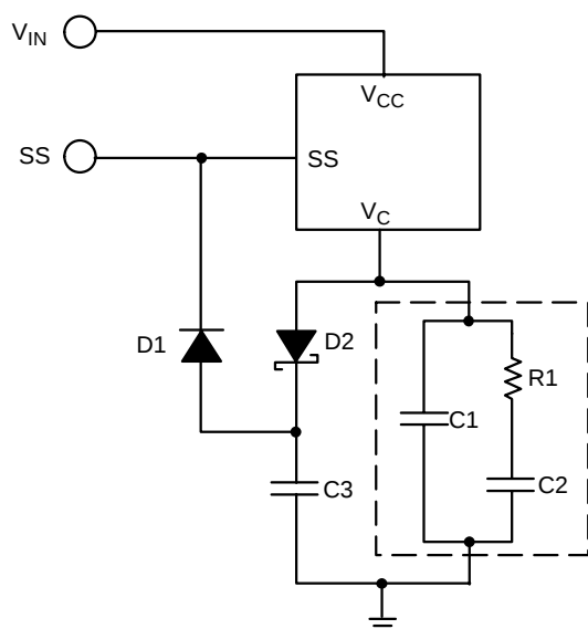
Figure 39. Soft-Start
