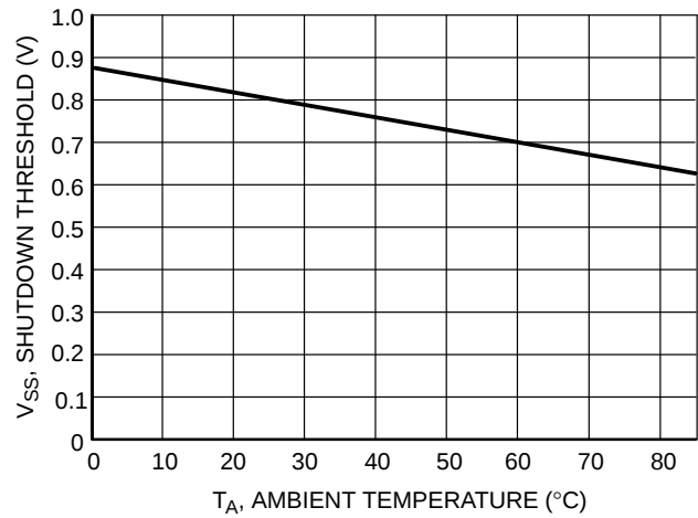
Figure 16. Shutdown Threshold versus Temperature
