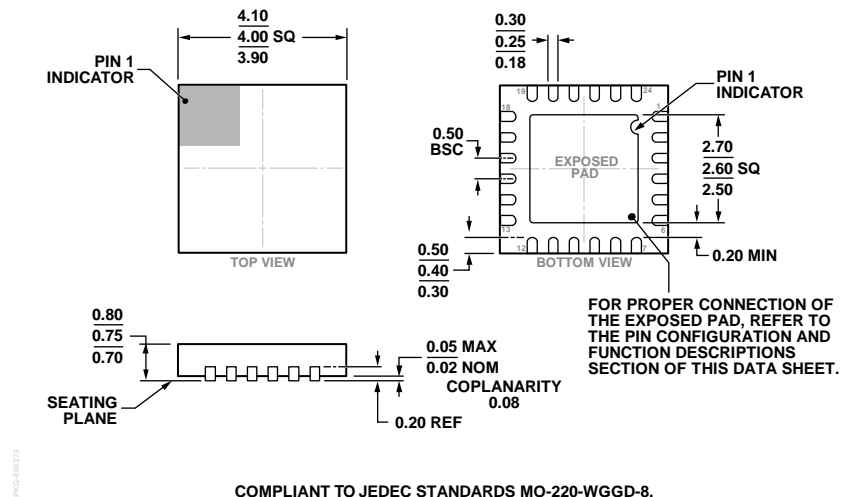
Figure 45. 24-Lead Lead-frame Chip Scale Package [LFCSP_WQ] (CP-24-15)
