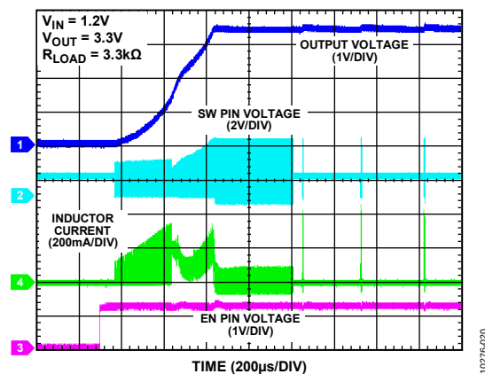
Figure 20. Startup, R_{LOAD} = 3.3\text{ k}\Omega
