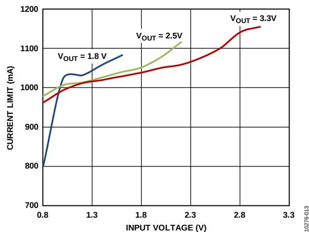
Figure 13. Switch Current Limit vs. Input Voltage
