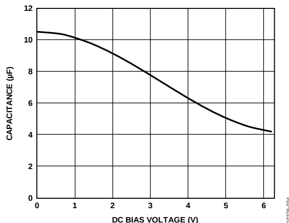
Figure 25. Typical Ceramic Capacitor Performance
