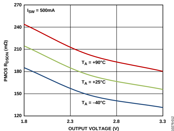
Figure 12. PMOS Drain-to-Source On Resistance
