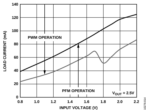
Figure 14. Auto Mode Transition Thresholds
