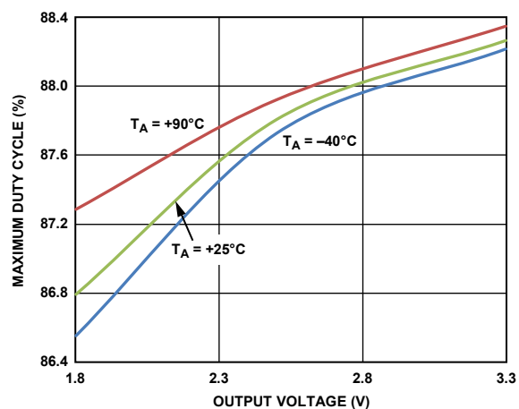
Figure 15. Maximum Duty Cycle vs. Output Voltage
