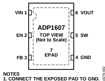
Figure 2. Pin Configuration
