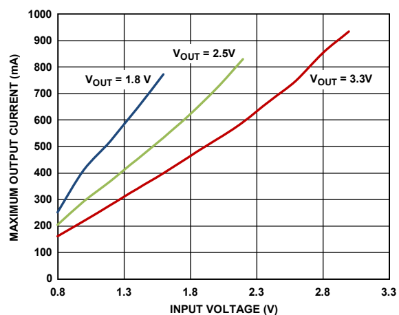
Figure 17. Maximum Output Current vs. Input Voltage
