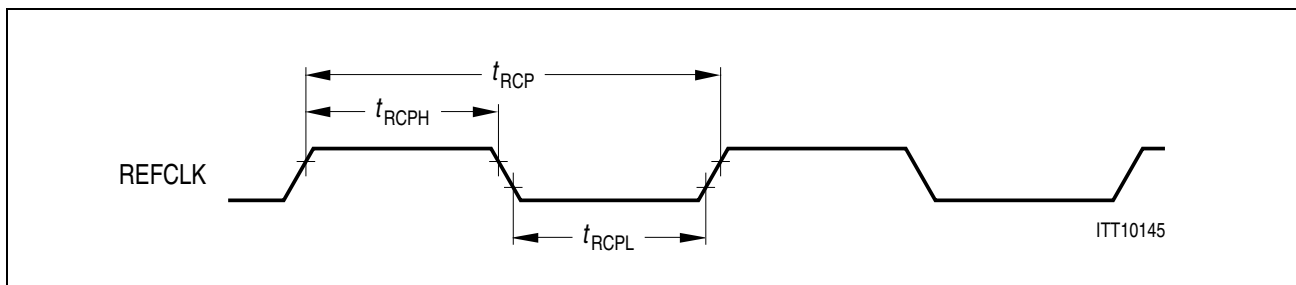
Figure 7-34 REFCLK Timing
