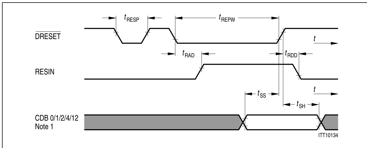
Figure 7-23 DRESET and RESIN timing
