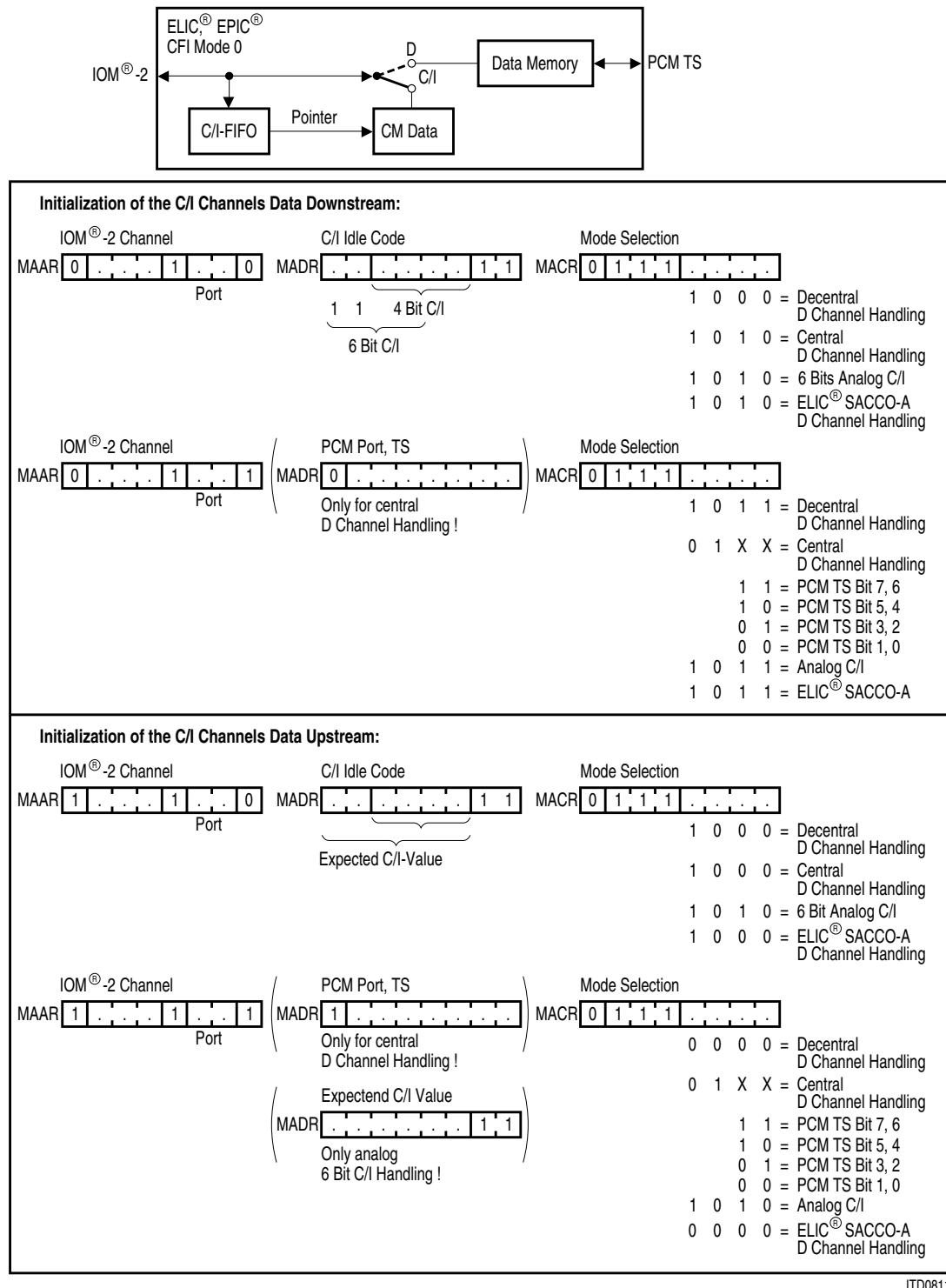
Figure 9-7 Preparing EPIC ® s C/I Channels (working sheet)
