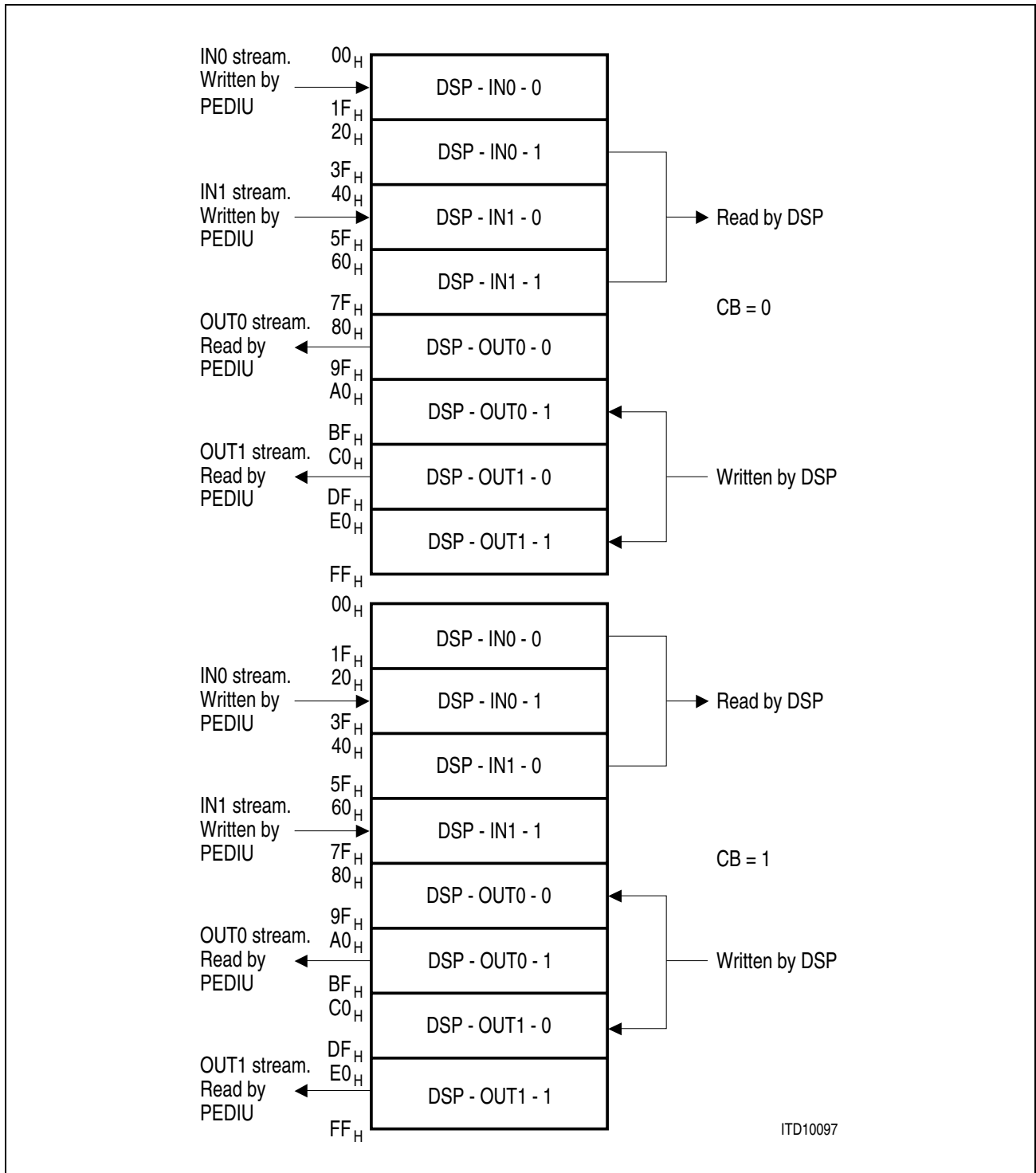
Figure 2-43 Connection between CB bit and Accesses to the Circular Buffer Blocks in PEDIU work Mode 0, 1 or 2
