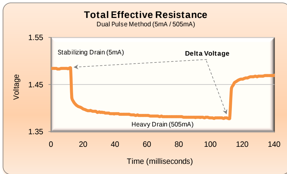
(fig. 9) 5 mA stabilization load / 505 mA pulse
