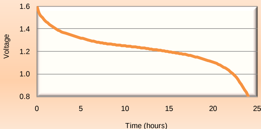
(fig. 12) AA/LR6 alkaline battery being discharged at 100mA to a 0.8 volt cutoff
