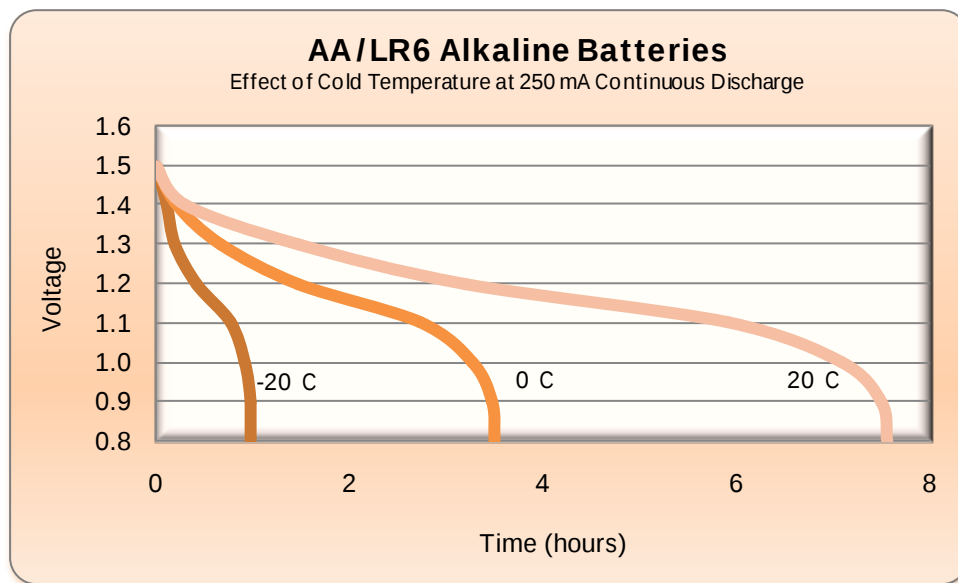
(fig. 5) Temperature impact on battery performance
