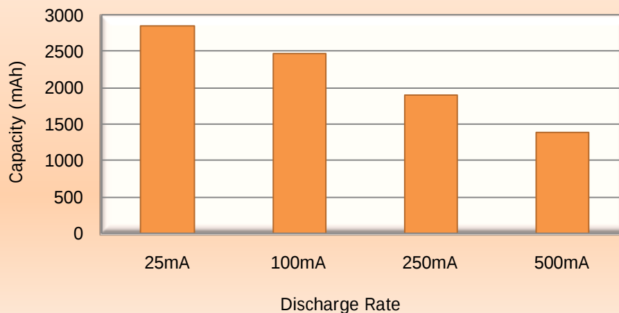
(fig. 13) AA/LR6 alkaline battery capacity to 0.8 volts
