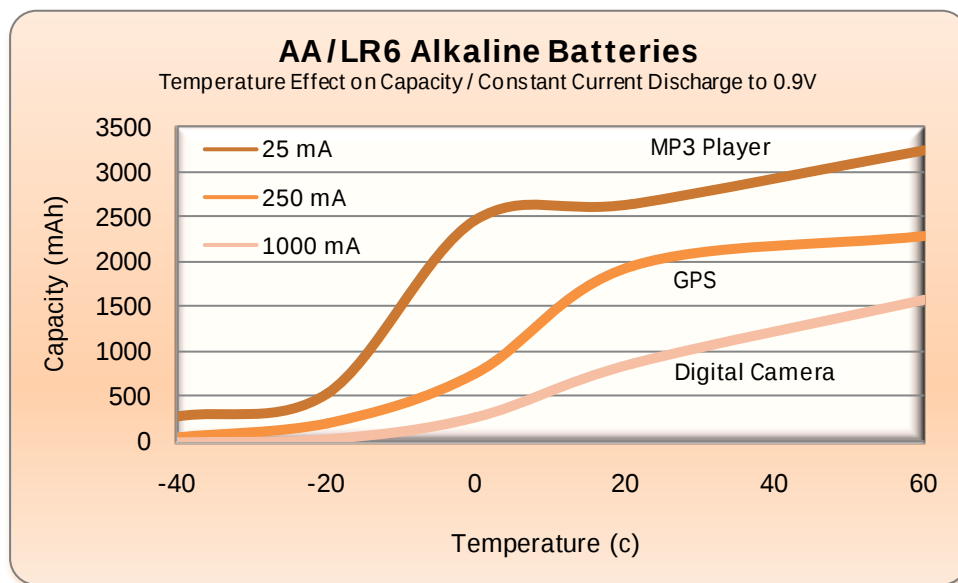
(fig. 6) Temperature Effect on Capacity
