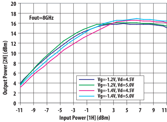
Figure 7. 2H Output Power Vs Input Power @ F_{out}=8\text{GHz}
