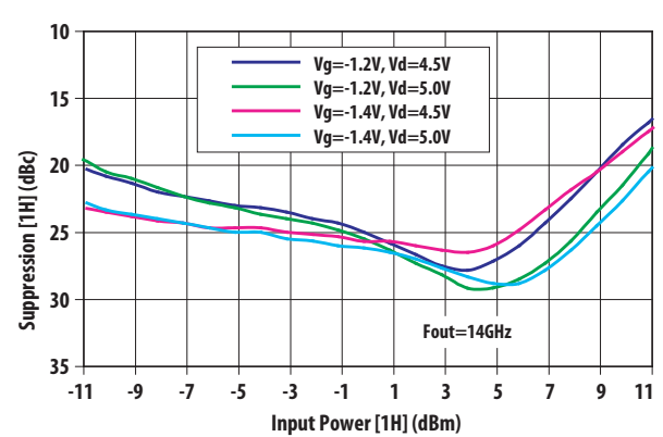
Figure 12. Fundamental Supp. Vs Input Power @ F_{out}=14\text{GHz}
