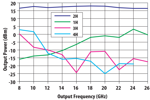
Figure 1. Output Power vs. Output Freq. @ P_{in} = +3\text{dBm}
