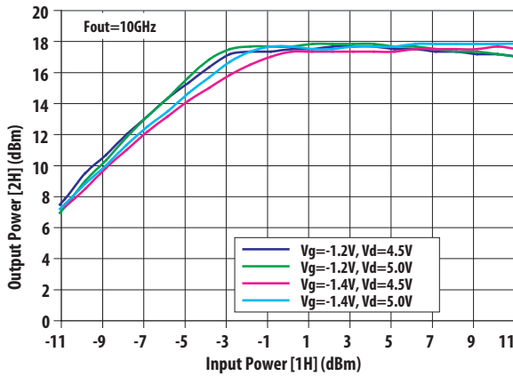
Figure 9. 2H Output Power Vs Input Power @ F_{out}=10\text{GHz}
