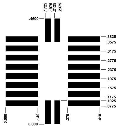
SM-20L PCB Pad Layout
