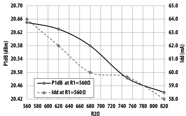
Figure 18. P1dB and Quiescent Current with different R1 [1]
