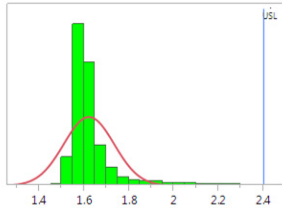
Figure 3. NF @ 1900 MHz; Nominal = 1.56 dB, USL = 2.4 dB
