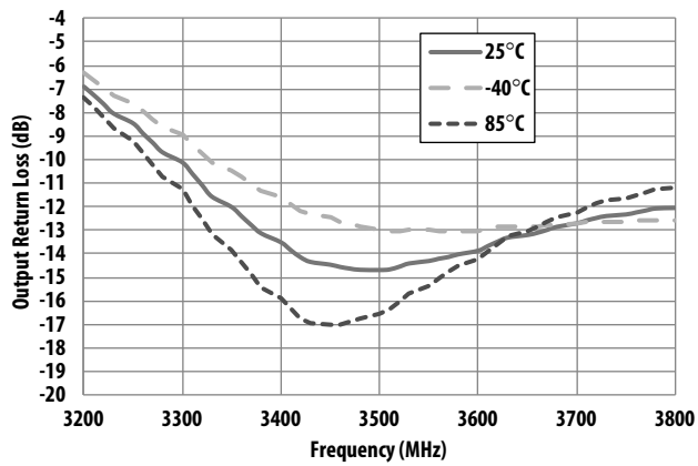
Figure 37. ORL vs Frequency and Temperature
