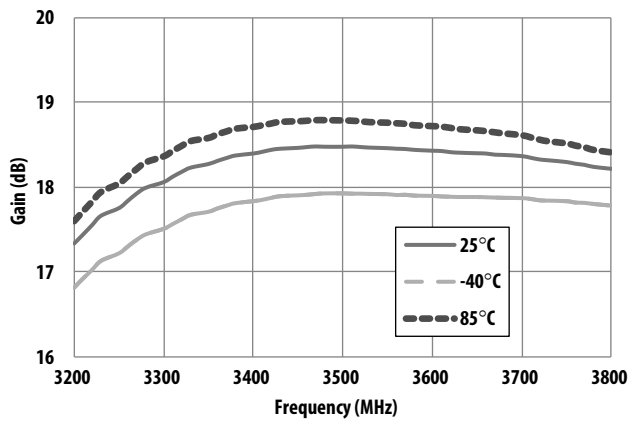
Figure 35. Gain vs Frequency and Temperature
