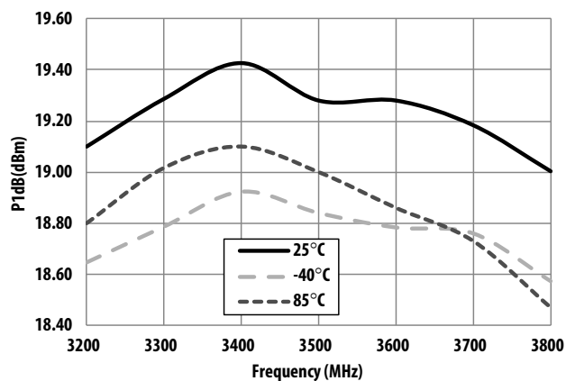
Figure 39. P1dB vs Frequency and Temperature
