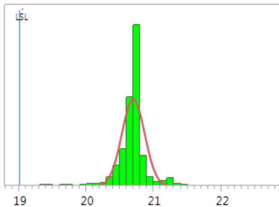
Figure 6. P1dB @ 1900 MHz; Nominal = 20.7 dBm, LSL = 19 dBm
