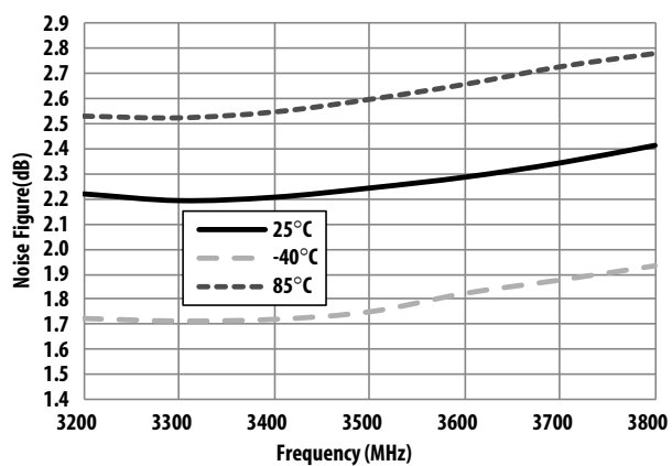
Figure 40. Noise Figure vs Frequency and Temperature
