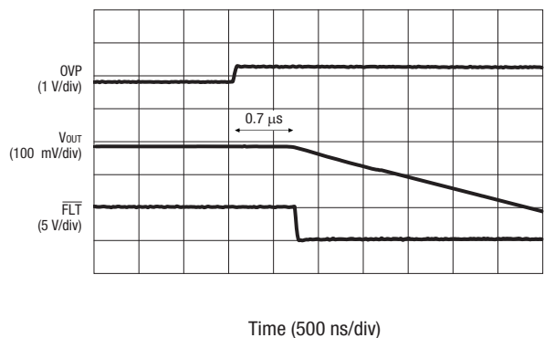
Figure 20. Over-Voltage Response Time ( V_{IN} = 5\text{ V} , OVP Transient from 0.8 V to 1.2 V)
