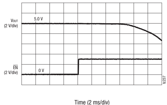
Figure 18. Turn Off Delay Time ( V_{IN} = 5\text{ V} , R_{OUT} = 10\ \Omega )
