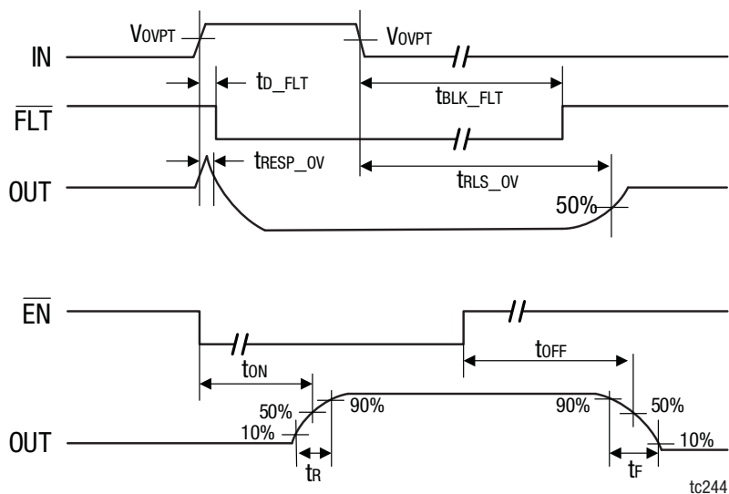
Figure 22. AAT4687 Timing Diagram
