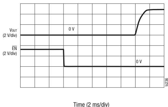
Figure 17. Turn On Delay Time ( V_{IN} = 5\text{ V} , R_{OUT} = 10\ \Omega )
