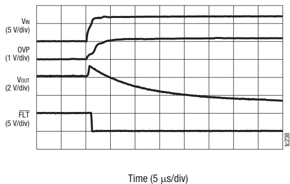
Figure 24. Typical Over-Voltage Response Time
