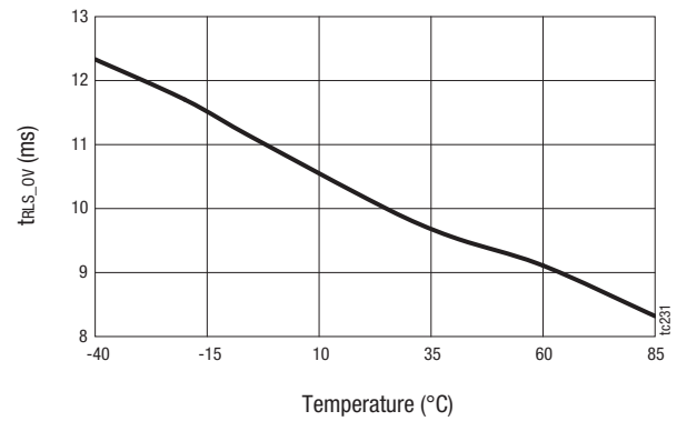
Figure 12. Over-Voltage Release Time vs Temperature ( V_{\text{IN}} = 5 \text{ V} , C_{\text{OUT}} = 1 \mu\text{F} , R_{\text{OUT}} = 10 \Omega )
