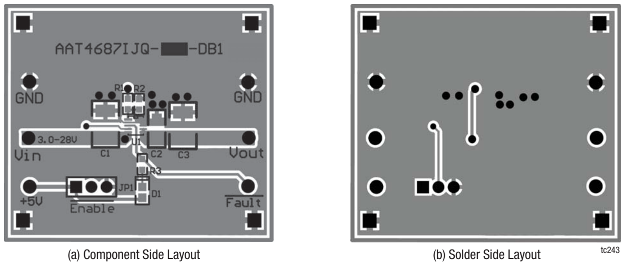
Figure 27. AAT4687 Evaluation Board Layer Details
