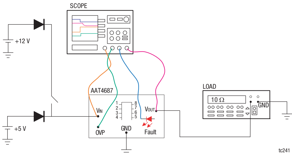
Figure 23. Over-Voltage Protection Response Time Test Circuit
