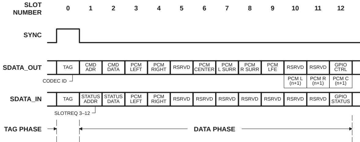
Figure 6. AC'97 Standard Bidirectional Audio Frame Basic Mode (Two-Channel)
