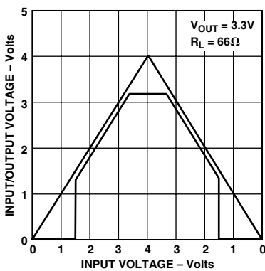
TPC 8. Power-Up/Power-Down
