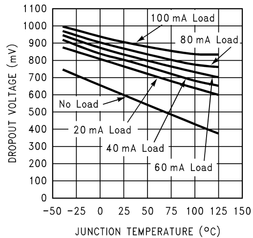
Dropout Voltage vs Junction Temperature
