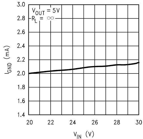
Ground Pin Current vs Input Voltage
