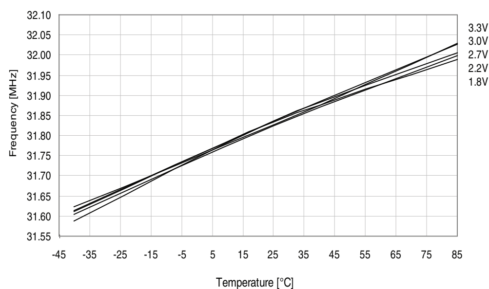
Figure 33-211. 32MHz internal oscillator frequency vs. temperature. DPLL enabled, from the 32.768kHz internal oscillator.
