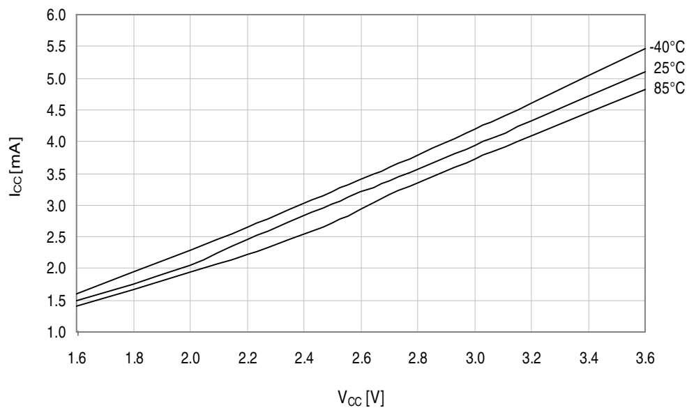
Figure 33-224. Active mode supply current vs. V_{CC} . f_{SYS} = 32\text{MHz} internal oscillator prescaled to 8\text{MHz} .
