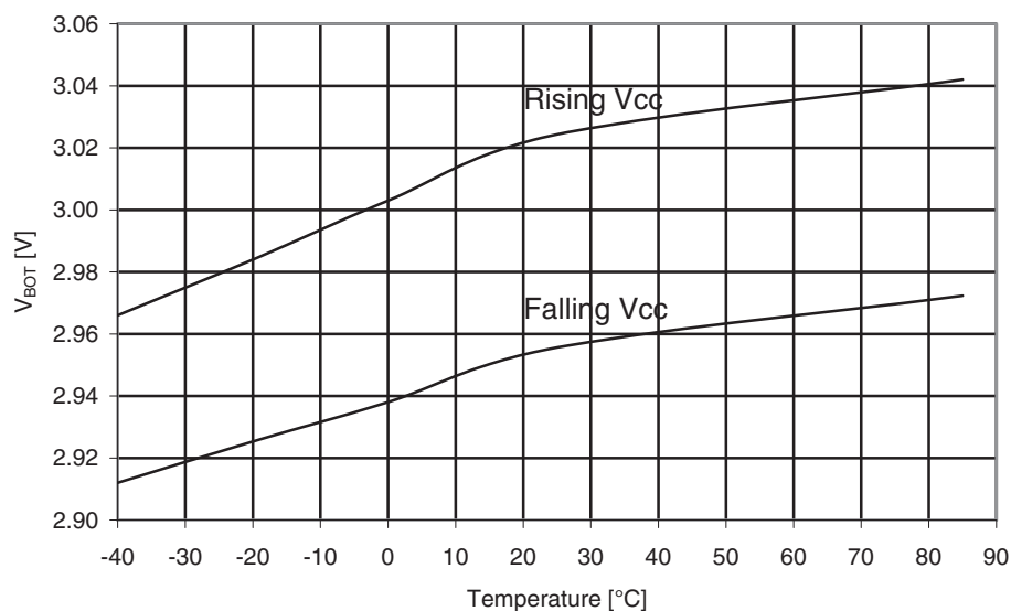
Figure 33-33. BOD thresholds vs. temperature. BOD level = 2.9V.
