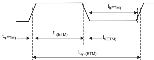
Figure 4-22. ETMTRACECLKOUT Timing
