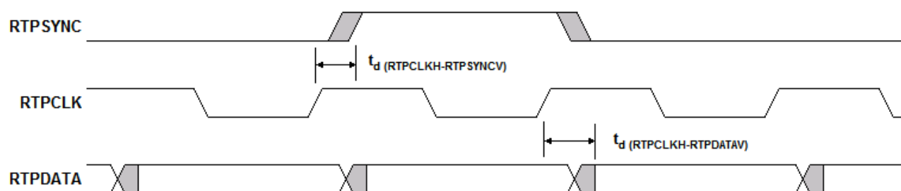
Figure 4-25. RTPDATA Timing
