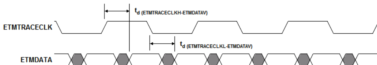
Figure 4-23. ETMDATA Timing
