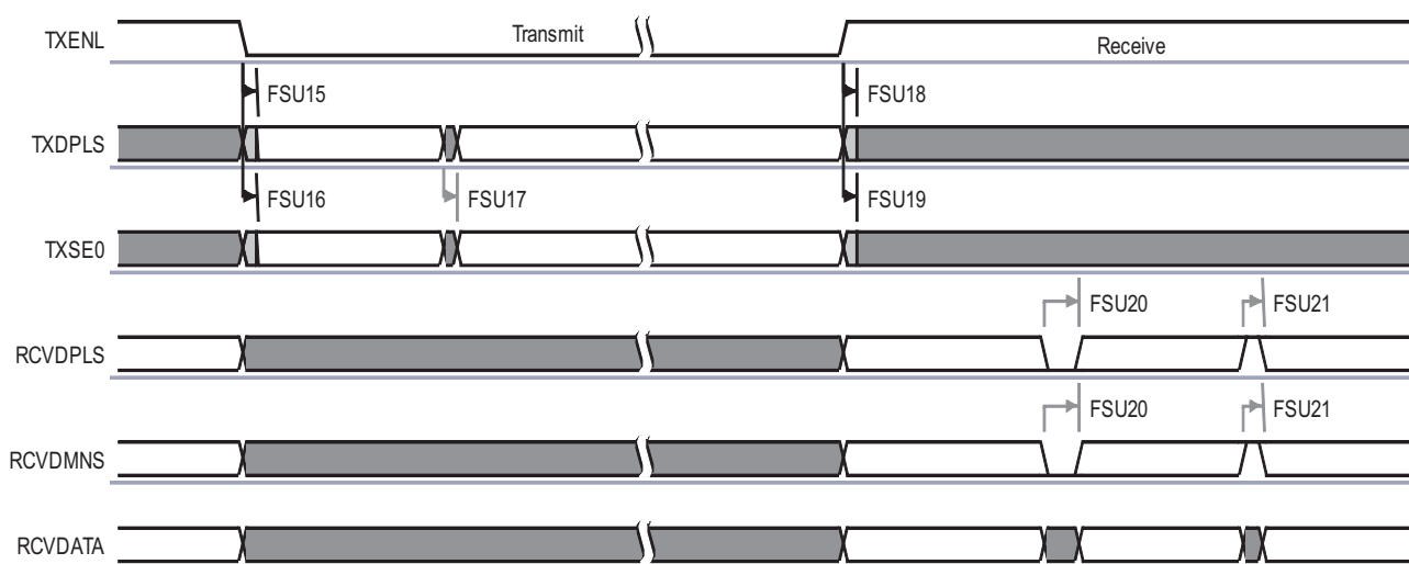
Figure 5-22. Full-Speed USB Interface – Transmit and Receive Modes
