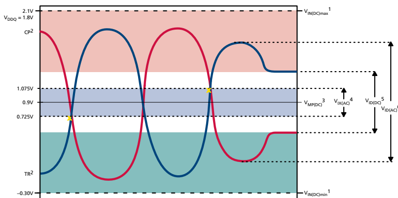
Figure 13: Differential Input Signal Levels
