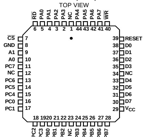
82C55A (PLCC)
