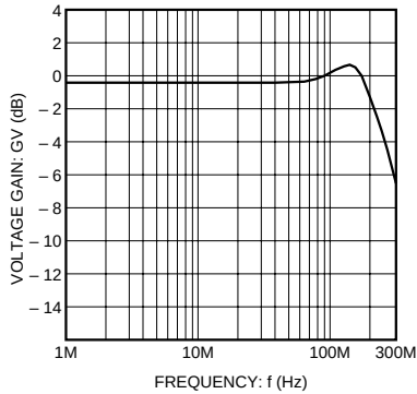
Fig. 4 Frequency characteristics
