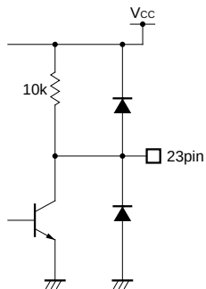
Signal detector output
