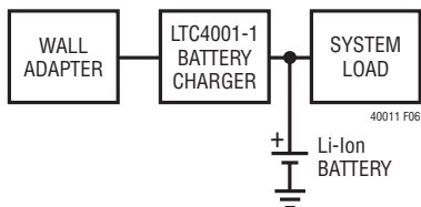
Figure 6. Typical Application
