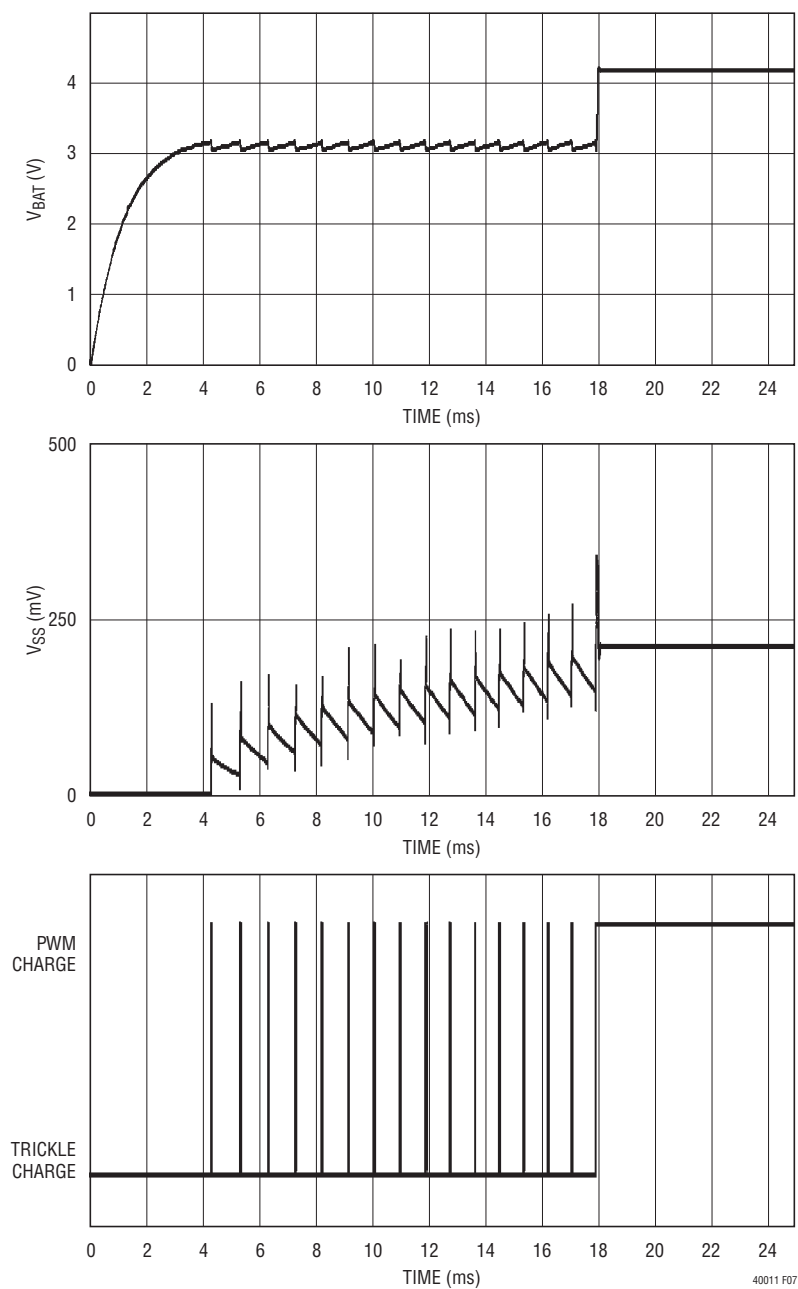
Figure 7. Battery-Less Start-Up
