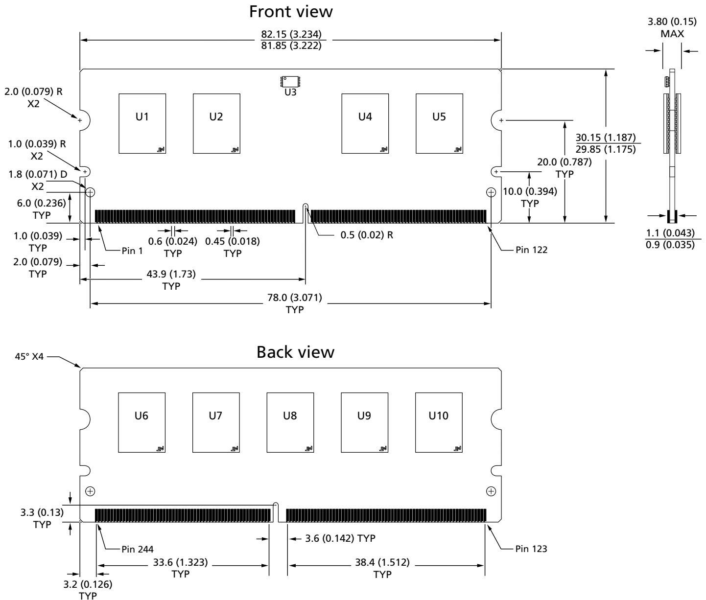
Figure 3: 244-Pin DDR3 Mini-UDIMM (MO-244)
