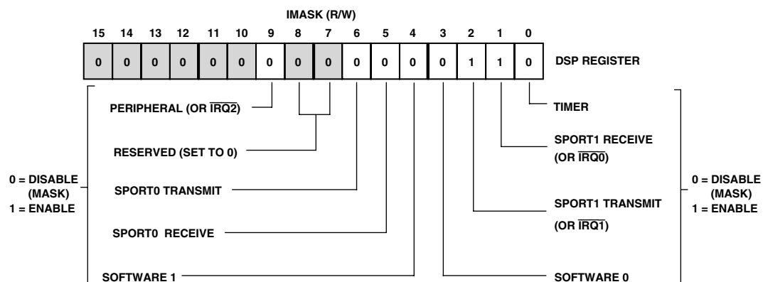
Figure 23. Configuration of ADMC331 Registers
