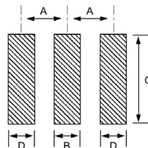
Figure 2) Land Pattern
