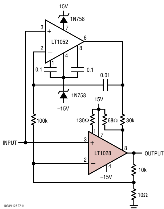
Chopper-Stabilized Amplifier
