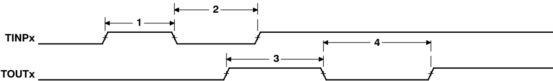
Figure 57. Timer Timing
