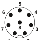
Plug, 8-pos.
