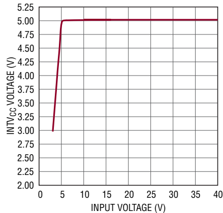
INT VC Line Regulation
