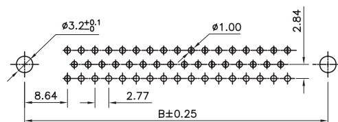
P.C. Board Layout (50 Positions)
