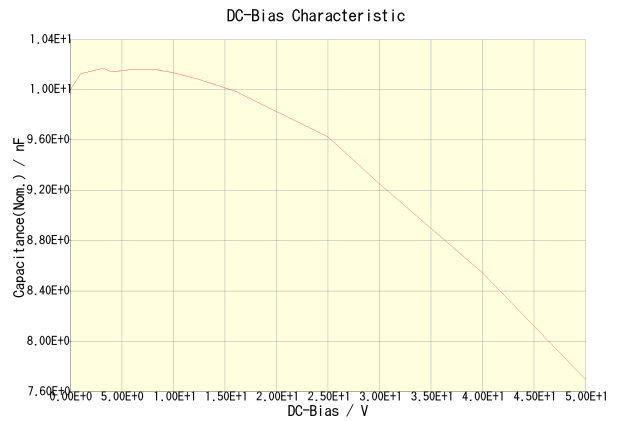
CKCA43X7R1H103M100AA
