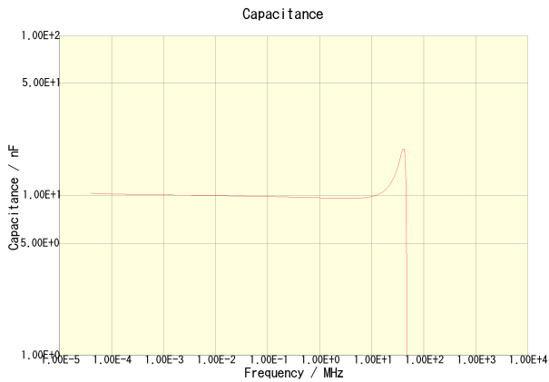
CKCA43X7R1H103M100AA
