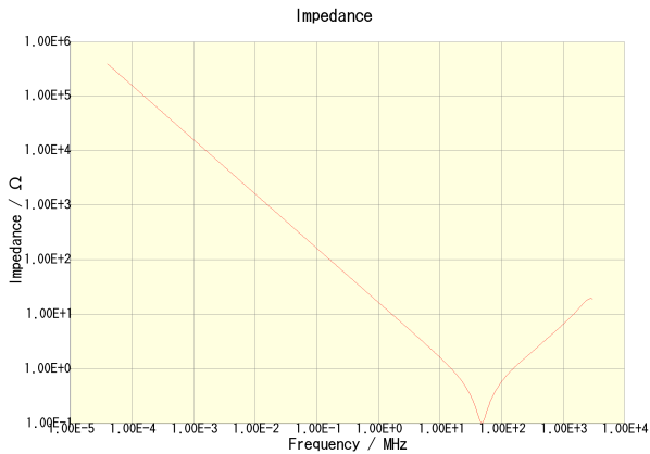
CKCA43X7R1H103M100AA
