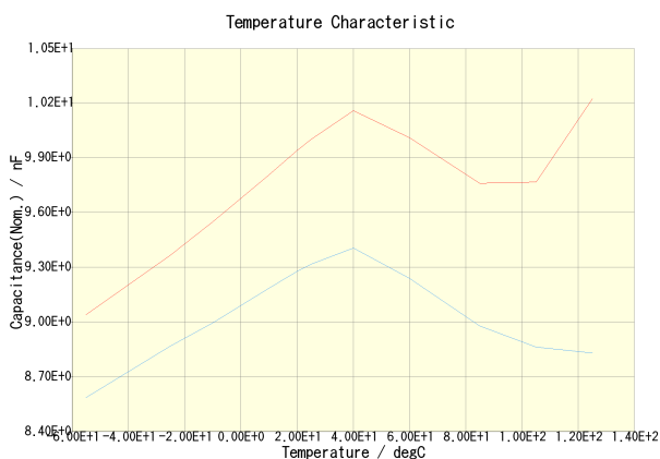
CKCA43X7R1H103M100AA(DC Bias = 0V) CKCA43X7R1H103M100AA(DC Bias = 25V)
