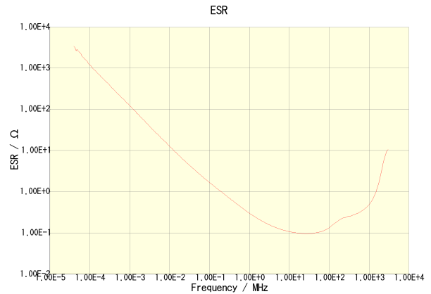
CKCA43X7R1H103M100AA
