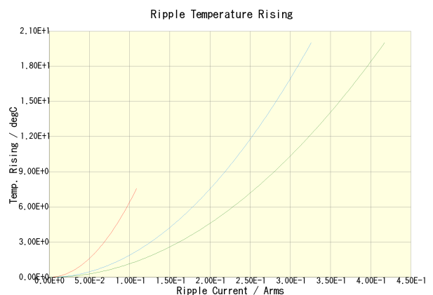
CKCA43X7R1H103M100AA(100kHz) CKCA43X7R1H103M100AA(500kHz) CKCA43X7R1H103M100AA(1MHz)
