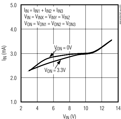
TOTAL SUPPLY CURRENT vs. INPUT VOLTAGE
