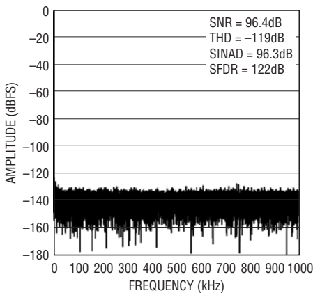
32k Point FFT f_S = 2\text{Msps} , f_{IN} = 2\text{kHz}
