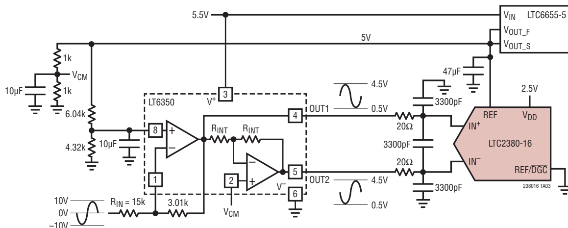
LT6350 Configured to Accept a \pm 10V Input Signal While Running Off of a Single 5.5V Supply When Digital Gain Compression Is Enabled in the LTC2380-16
