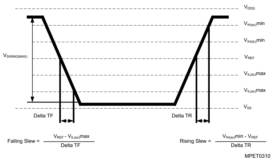
FIGURE 4 Single-ended AC Input Test Conditions Diagram
