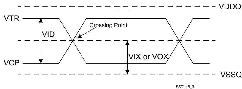
FIGURE 5 Differential DC and AC Input and Output Logic Levels Diagram
