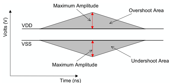
AC Overshoot / Undershoot Diagram for Address and Control Pins
