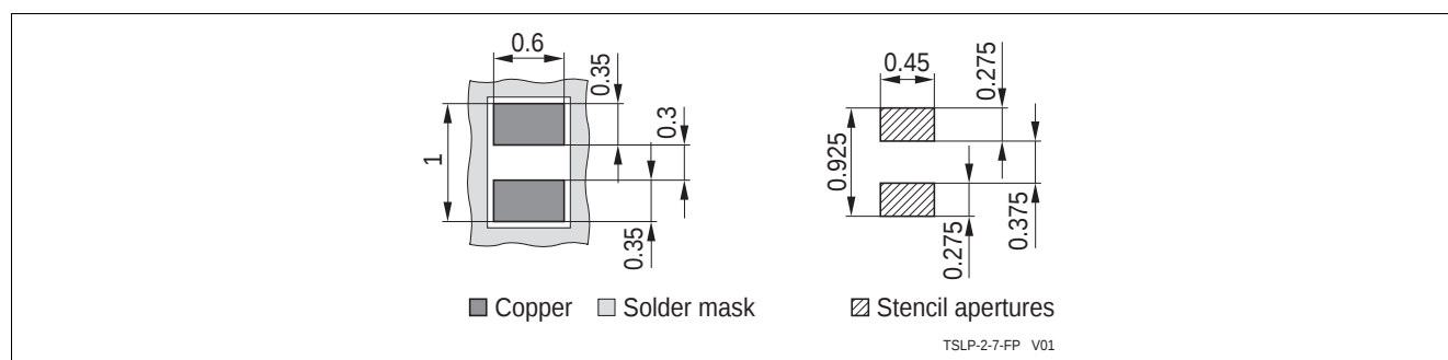
Figure 13 PG-TSLP-2-17: Footprint
