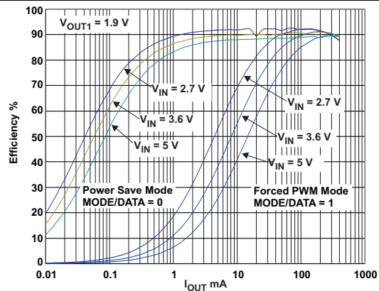
Figure 22. Efficiency TPS62404 VOUT1 = 1.9V, DEF_1 = HIGH
