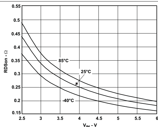
Figure 4. R_{DSon} PMOS vs V_{IN}
