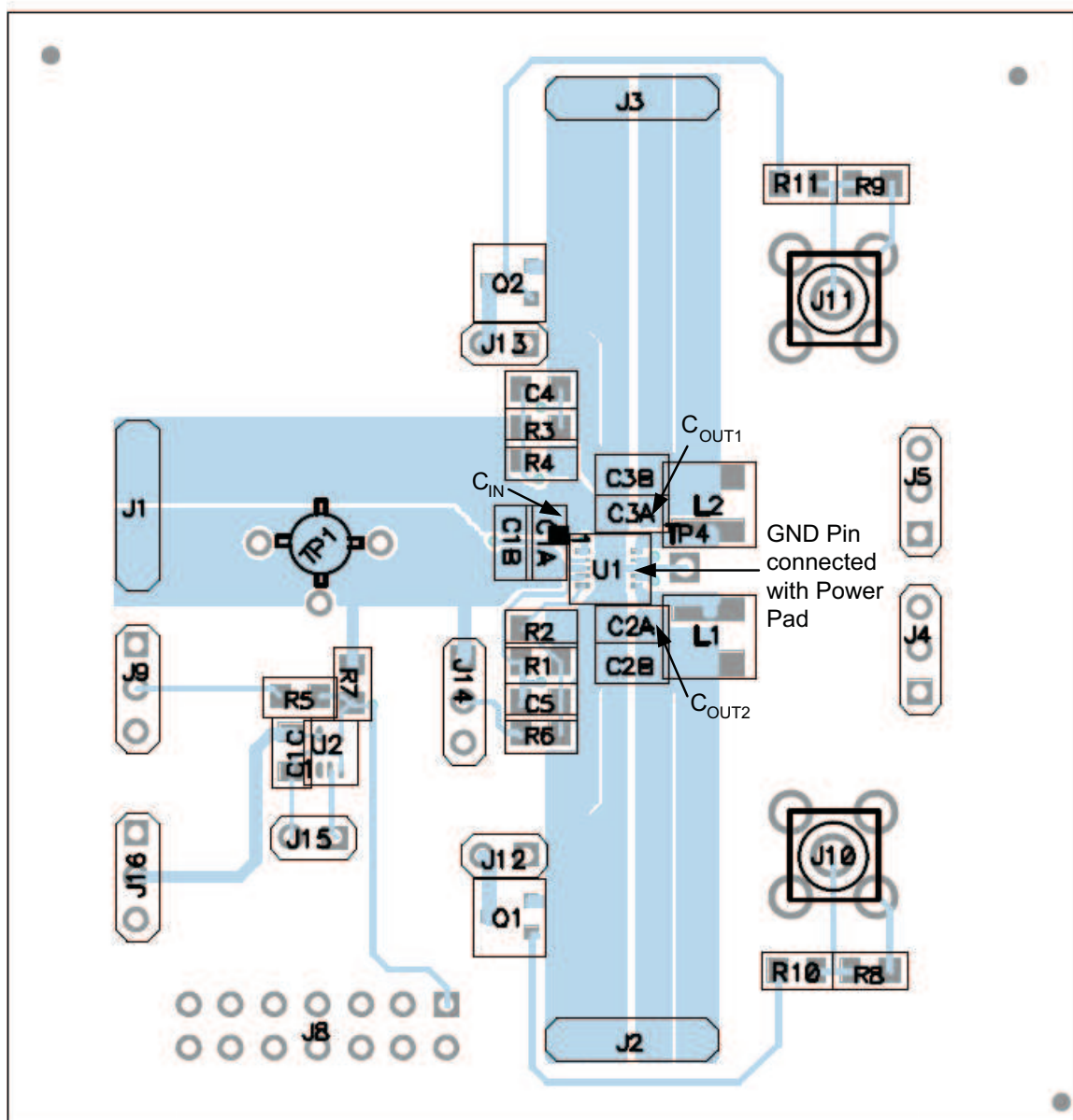
Figure 49. PCB Layout
