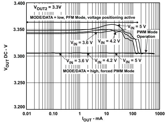
Figure 26. DC Output Accuracy V_{OUT2} = 3.3V
