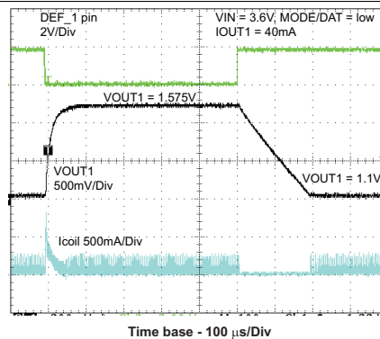
Figure 47. TPS62401DEF1_PIN Function For Output Voltage Selection
